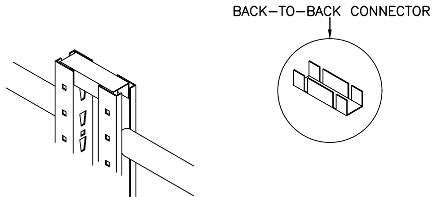
DETAIL N
