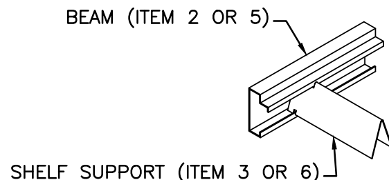
DETAIL H
