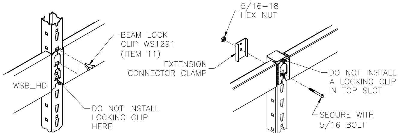
DETAIL P
