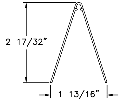
Standard Duty Shelf Support (Item 3)
